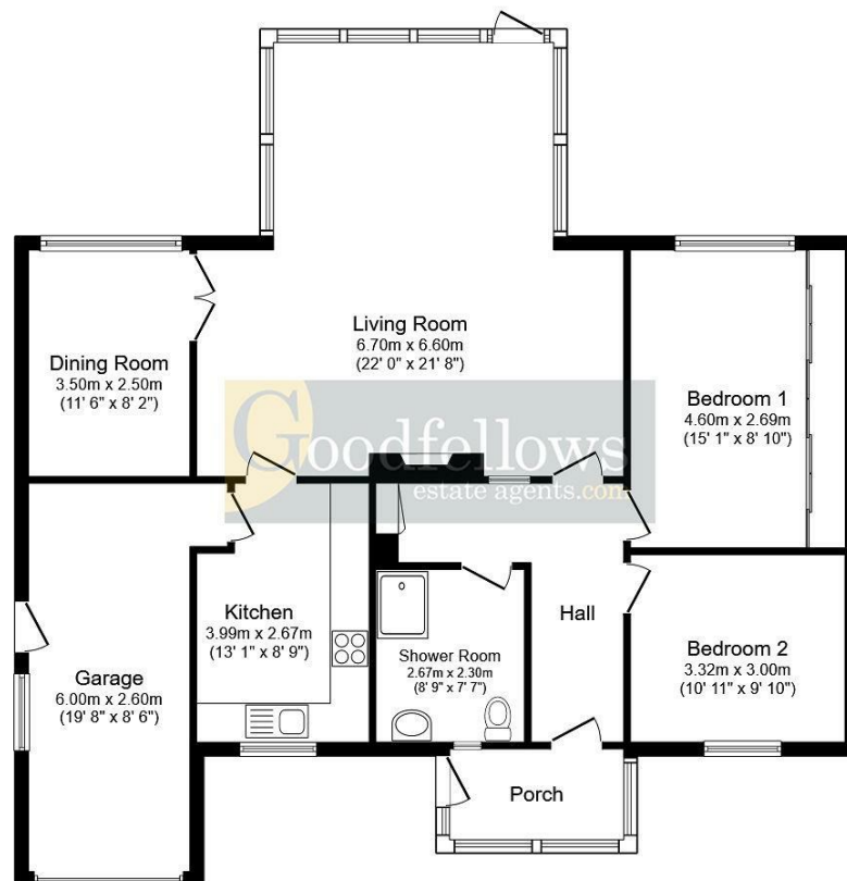
Floor Plan
